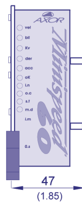
11 TE Encoder Feedback version (Optional)
